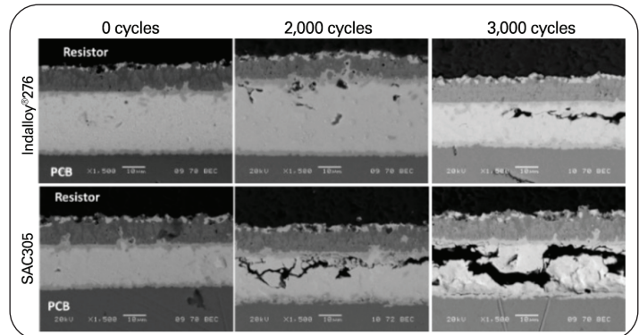
Figure 9. Backscattered electron SEM images of the cross sections of SMR0805 resistors on the ImSn surface finish after 0, 2,000, and 3,000 cycles under TCT -40°C/125°C.
