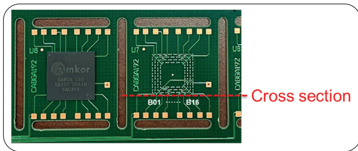
Figure 11. The fully populated CABGA192 PCB test board used in this study and the location where the cross sections were examined.
