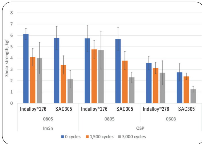
Figure 4. Shear strength of SMR0603 and SMR0805 resistors for SAC305 and Indalloy®276 alloys at 0, 1,500, and 3,000 cycles under TCT (-40°C/125°C).
