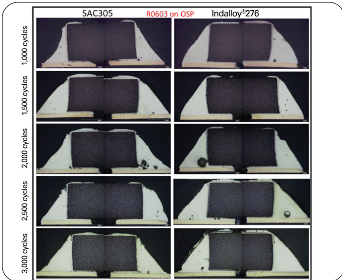
Figure 7. Cross-sectional optical micrographs of SMR0603 on the OSP surface finish after 1,000, 1,500, 2,000, 2,500, and 3,000 cycles under TCT -40°C/125°C.
