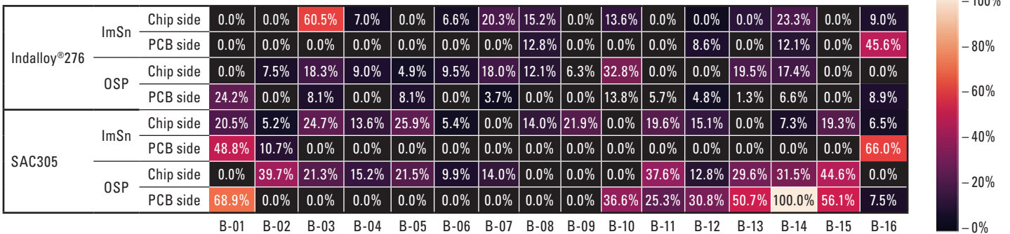
Figure 15. The crack ratio of each joint/ball at both the component side and PCB side in SAC305 and Indalloy®276 at 1,000, 1,600, and 3,000 cycles under TCT -40°C/125°C.
