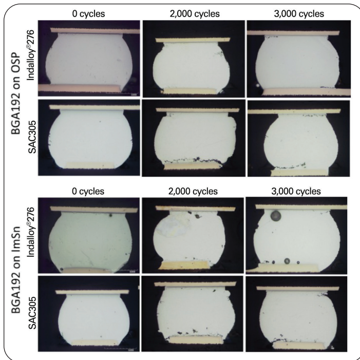
Figure 14. Comparison of the cross sections of corner joints from BGA192 of SAC305 and Indalloy®276 at 0, 2,000, and 3,000 cycles under -40^{\circ}\text{C}/125^{\circ}\text{C} .
