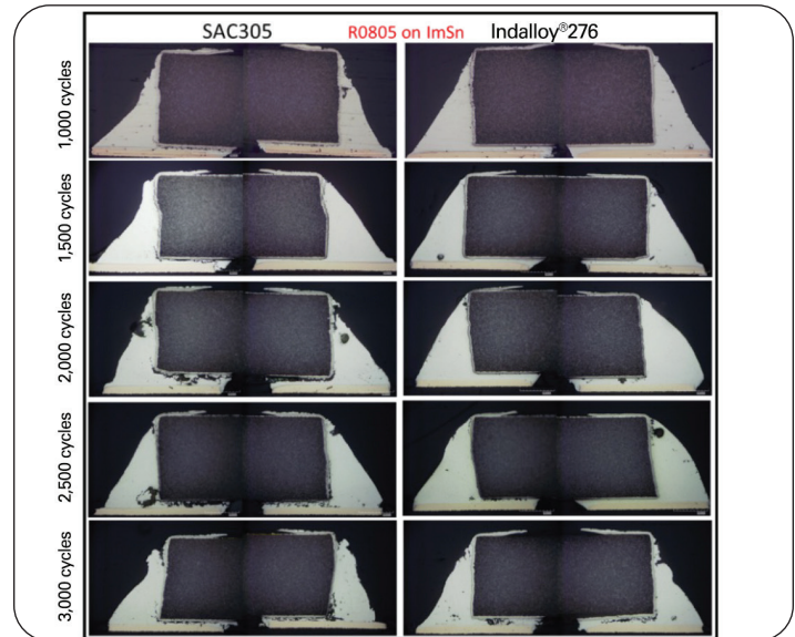
Figure 6. Cross-sectional optical micrographs of SMR0805 on the ImSn surface finish after 1,000, 1,500, 2,000, 2,500, and 3,000 cycles under TCT -40°C/125°C.
