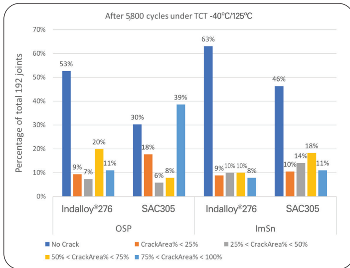
Figure 17. Statistics of the crack area per joints in SAC305 and Indalloy®276 after 5,800 cycles under TCT -40°C/125°C.
