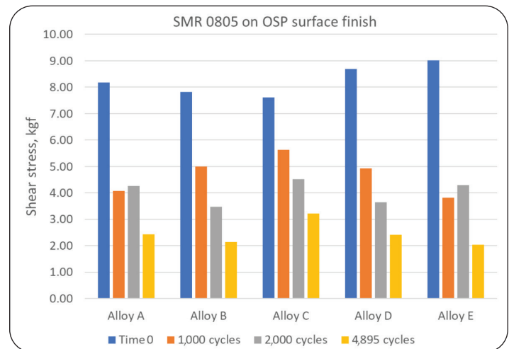
Figure 3. The shear strength of Sn/3.2Ag/0.7Cu/xSb alloys after 1,000, 2,000, and 4,895 cycles of thermal cycling at -40°C / 125°C.
