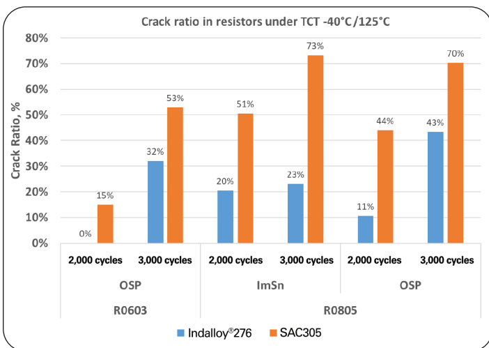
Figure 8. The crack ratio in resistors of SAC305 and Indalloy®276 after 2,000 and 3,000 cycles under TCT -40°C/125°C.
