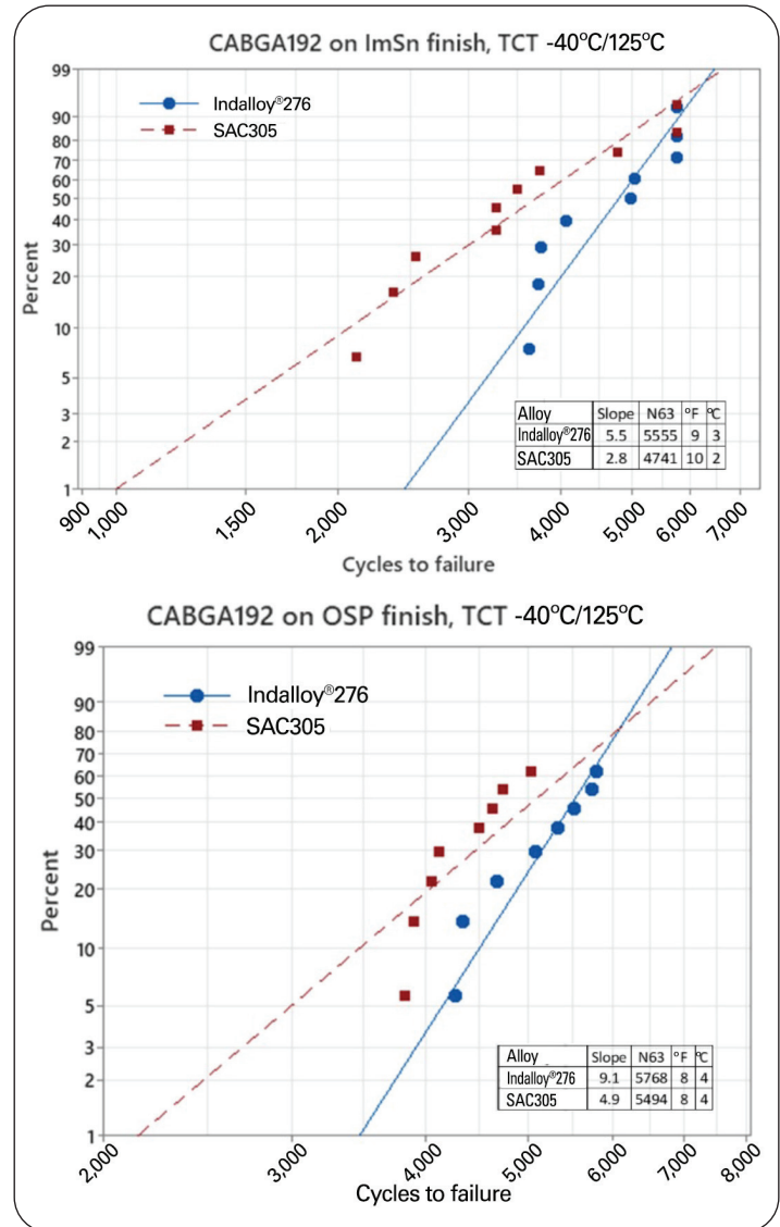
Figure 12. Right-censored Weibull plots for SAC305 and Indalloy®276 tested with the CABGA192 on ImSn and OSP surface finishes under TCT -40°C/125°C.
