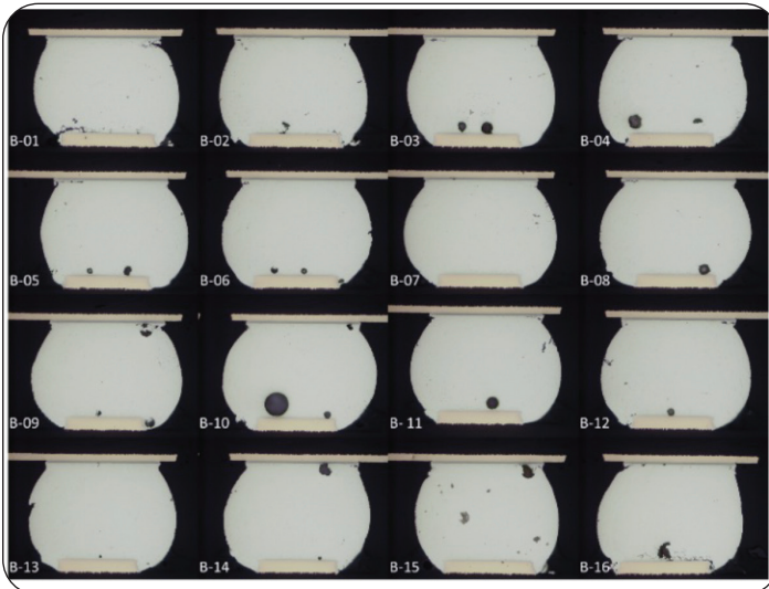
Figure 13. The cross section of CABGA192 of SAC305 on the ImSn surface finish after 3,000 cycles under -40^{\circ}\text{C}/125^{\circ}\text{C} .
