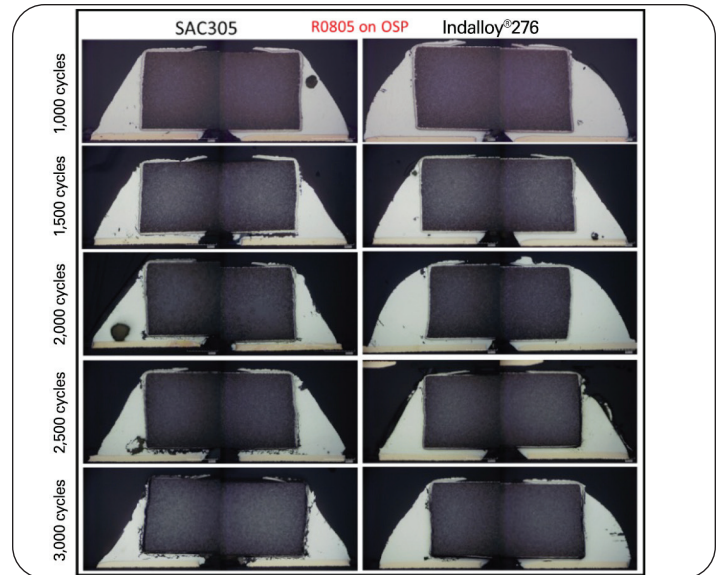
Figure 5. Cross-sectional optical micrographs of SMR0805 on the OSP surface finish after 1,000, 1,500, 2,000, 2,500, and 3,000 cycles under TCT -40°C/125°C.
