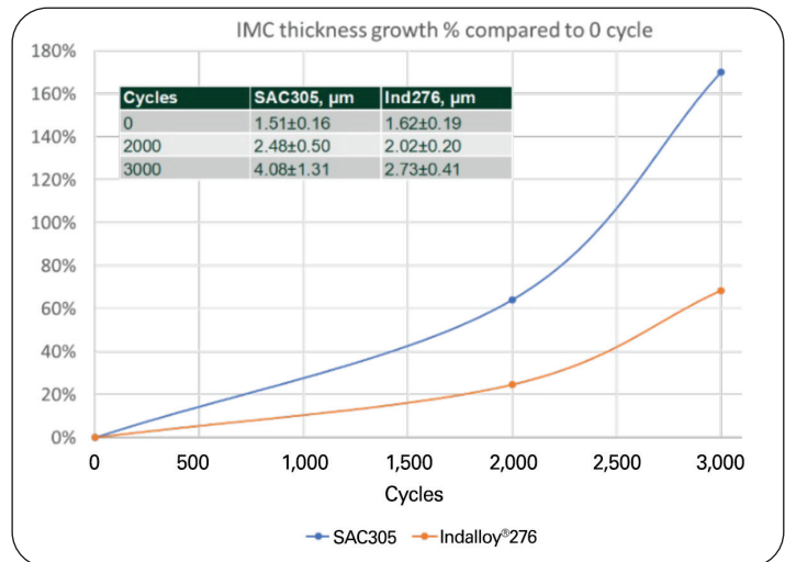
Figure 10. The IMC layer thickness growth rate (compared to 0 cycle) in SMR0805 resistors of SAC305 and Indalloy®276 at 2,000 and 3,000 cycles under TCT -40°C/125°C.
